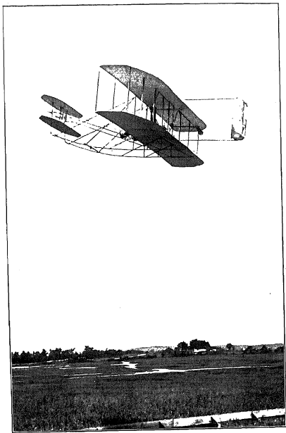
FIG. 21 WRIGHT BROTHERS' AEROPLANE, FORT MYER, VA., SEPTEMBER 12, 1908. TIME OF FLIGHT, 1 HR., 14 MIN., 20 SEC.
