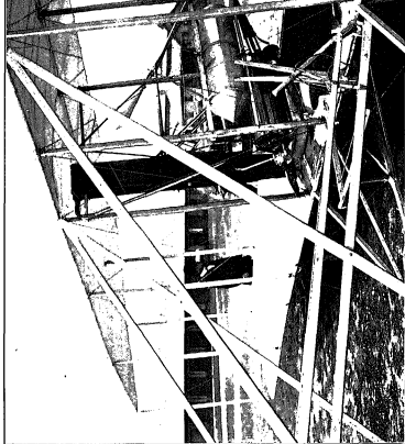
FIG. 14 WRIGHT BROTHERS' AEROPLANE; DETAILS OF CONSTRUCTION
